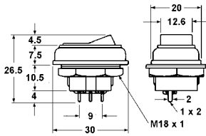
Round 18mm diameter mounting hole 6A @ 125VAC
