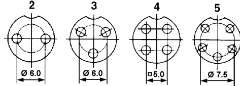
Pin Layout
